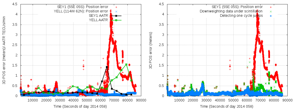
Figure 1. Left hand plot shows the 3D error of Precise Point Positioning for two receivers affected by scintillation. Red color is for a receiver located at low latitude (SEY1). Blue color is for a receiver at high latitude YELL). The AATR values are shown in black and green, respectively. The right hand plot shows the 3D positioning error of the low latitude receiver SEY1. The effect, at the user domain, of undetected small cycle-slips due to the scintillation conditions is shown in red. The solution in green has been computed down-weighting in real-time the measurements of satellites affected by scintillation. The navigation error computed using an (off-line) reliable cycle-slip detector able to detect very small jumps (involving just 1 cycle of L1 or L2 carriers) is shown in blue.
